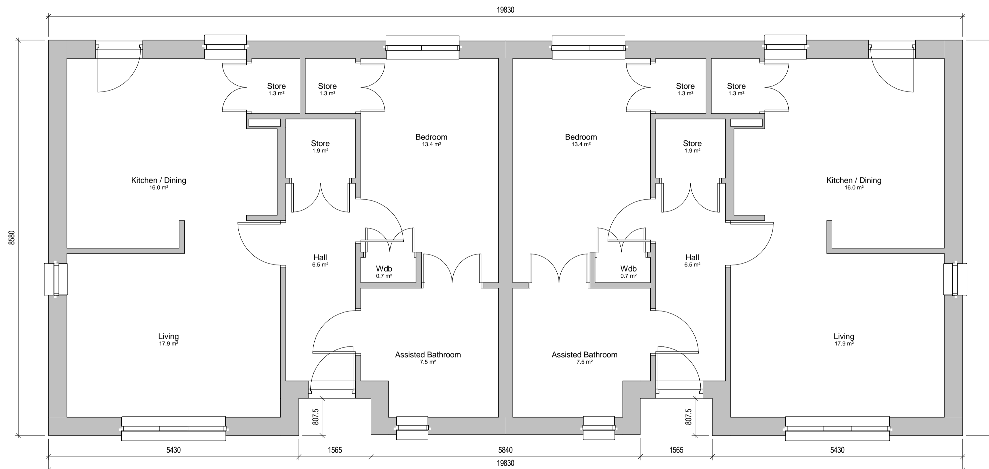
Gd. FLOOR PLAN 1Bed / 2Pers Bungalow HOUSE TYPE G (LH) GIFA 71.03m 2 STORAGE = 5.2m 2
