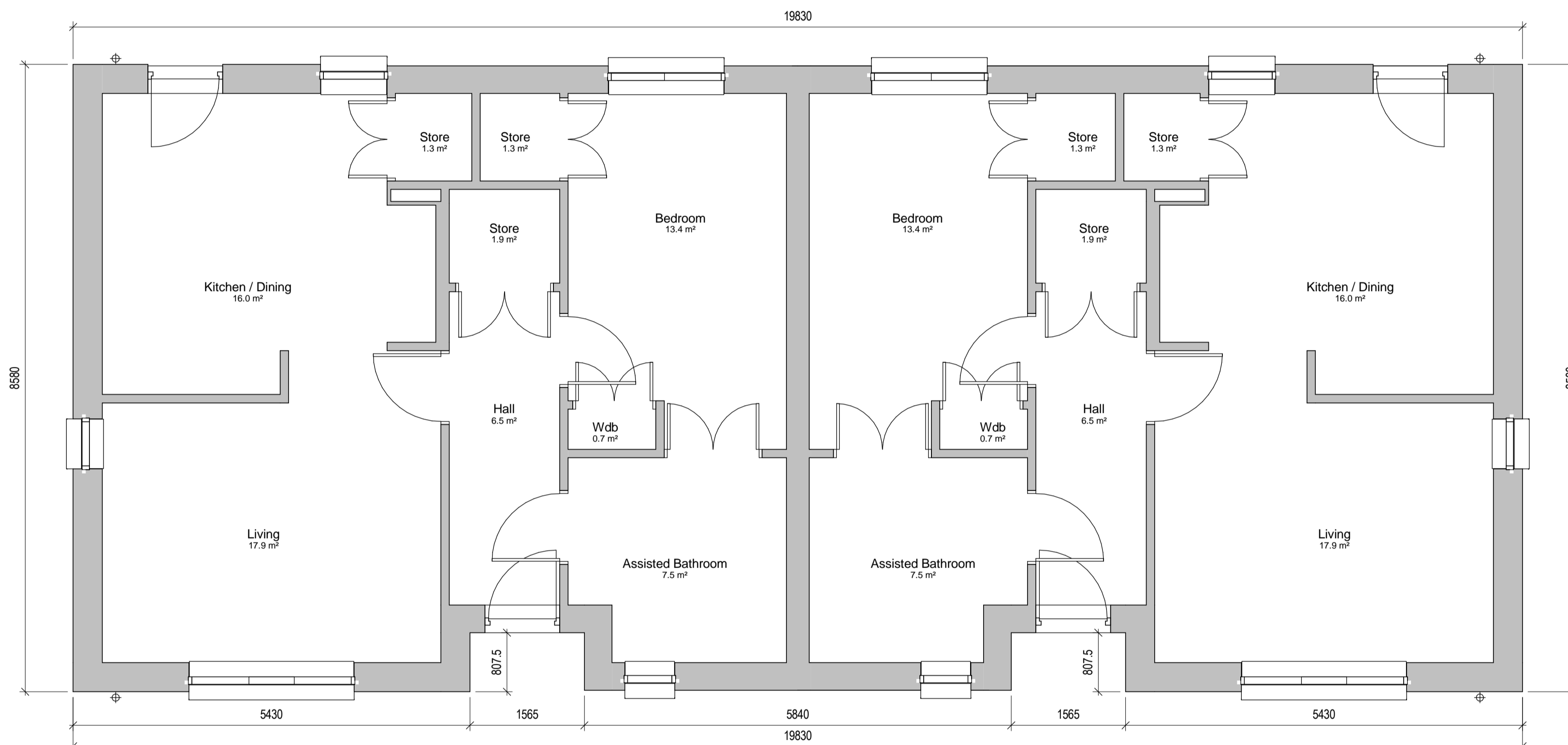
Gd. FLOOR PLAN 1Bed / 2Pers Bungalow HOUSE TYPE G (LH) GIFA 71.03m 2 STORAGE = 5.2m 2 Block 17 - Ground Floor Plan 1 : 50
